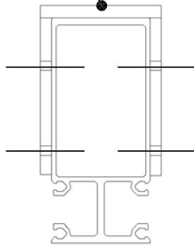
VERTICAL SECTION
