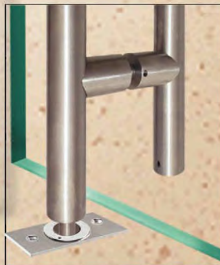
PL-FLOOR STRIKE 1 15/16" X 1 7/16" DUST PROOF STRIKE OPTION
