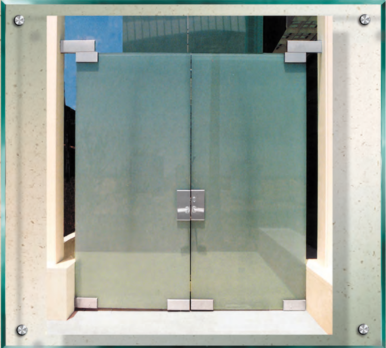
F Doors with custom centerlock/strike housing, Latchlock and electric strike.
