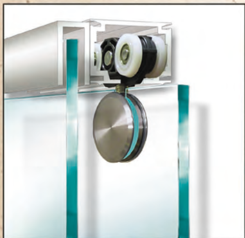
Top Hung Slider Door/Sidelite
