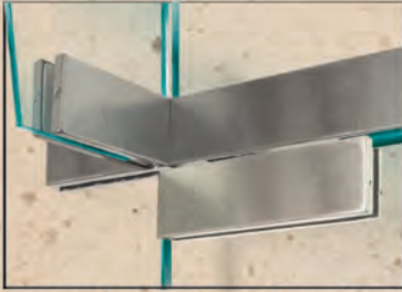
PD-TVS Custom Header TRANSOM/SL/FIN/PIVOT BRACKET 4 1/8" H / 8 1/2" W
