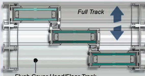
Flush Cover Head/Floor Track Inactive Sliding Guides
