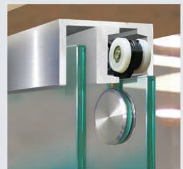
Top Hung Slider Door/Sidelite 2 3/8" Diameter Bracket
