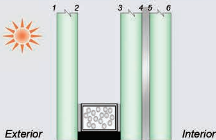
IG Unit Laminated Inboard
