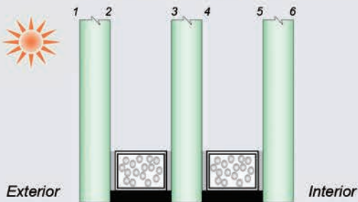
Triple-Glazed IG Unit
