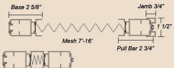
Finished Stack Width
