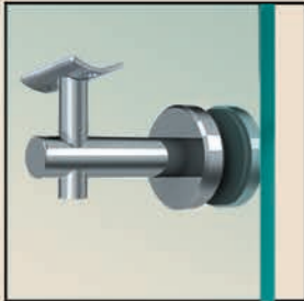
PL- HR20XEGPS Adjustable Glass Mount Bracket for 1 1/2" Dia Tubing
