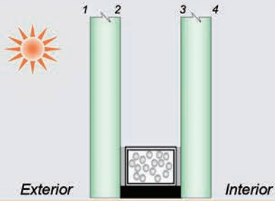
Double-Glazed IG Unit
