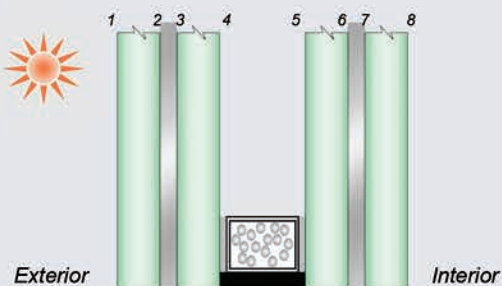
IG Unit Laminated Inboard/Outboard
