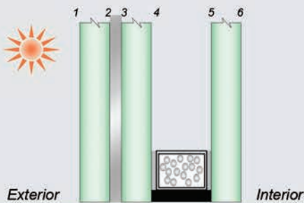
IG Unit Laminated Outboard
