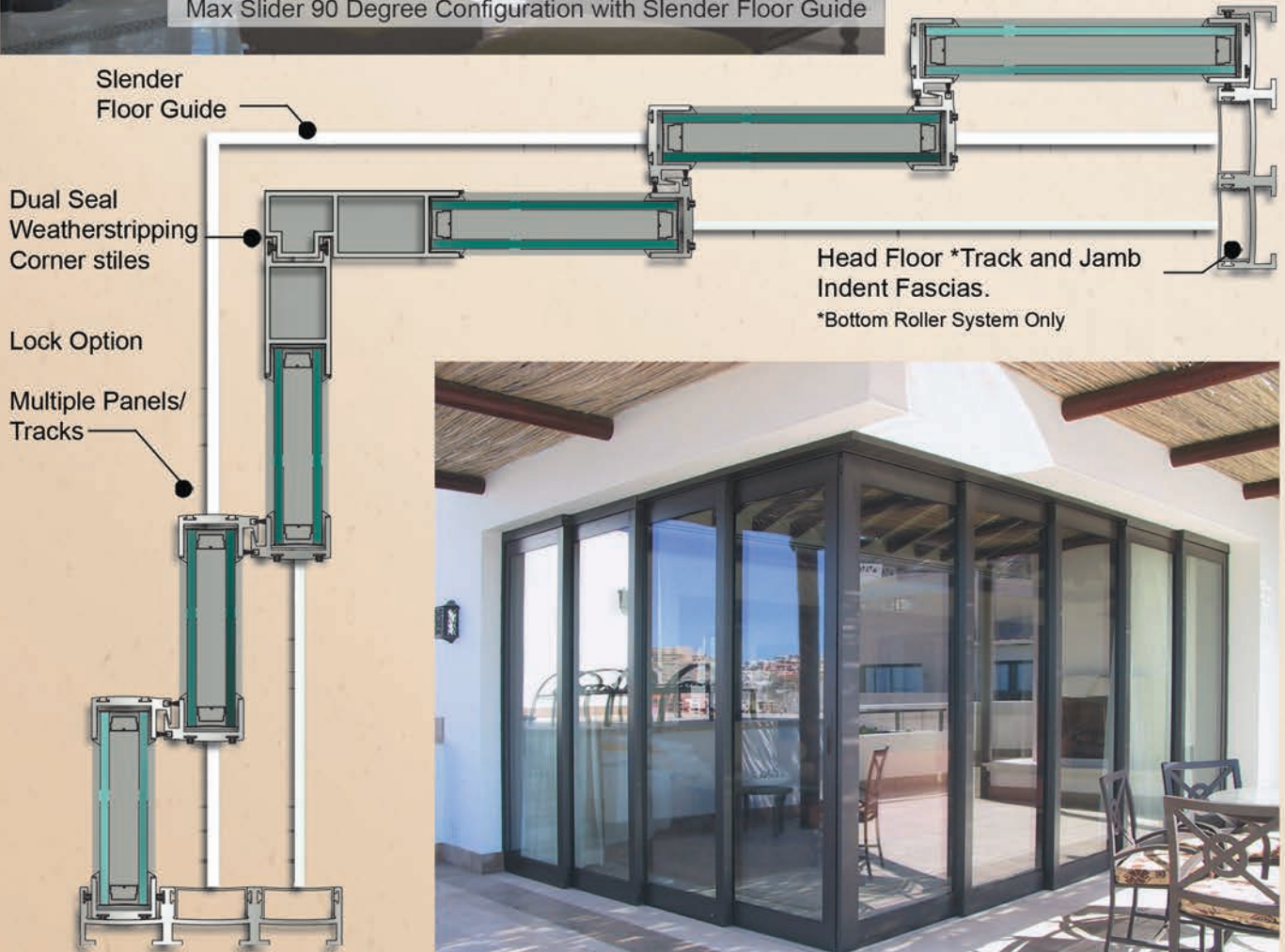
Max Slider 90 Degree Configuration with Slender Floor Guide
